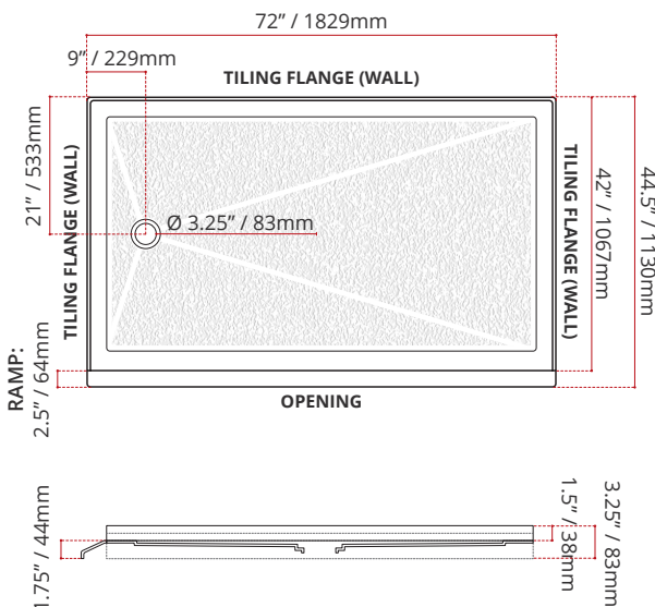
BSSTOD7242L1 (LEFT HAND DRAIN LOCATION)
