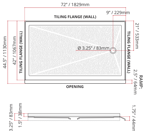
BSSTOD7242R1 (RIGHT HAND DRAIN LOCATION)
