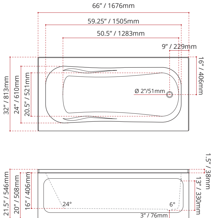
MODEL NUMBER : 4181 (RIGHT HAND DRAIN LOCATION)
