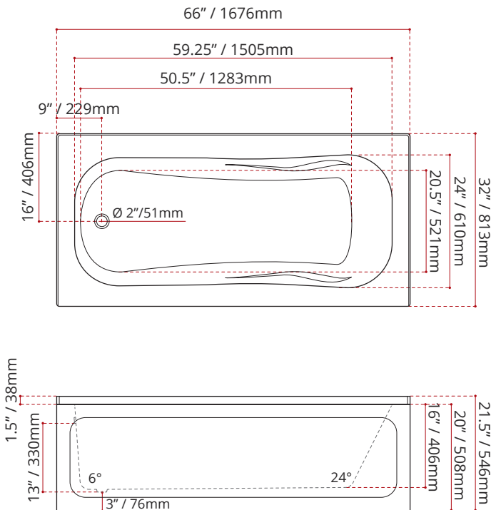
MODEL NUMBER : 4171 (LEFT HAND DRAIN LOCATION)
