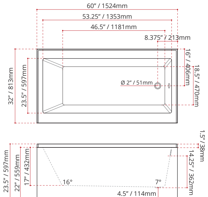
MODEL NUMBER : 2321 (RIGHT HAND DRAIN LOCATION)
