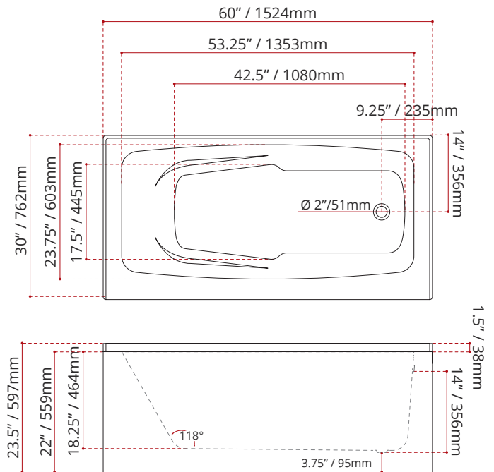
MODEL NUMBER : 5215 (RIGHT HAND DRAIN LOCATION)
