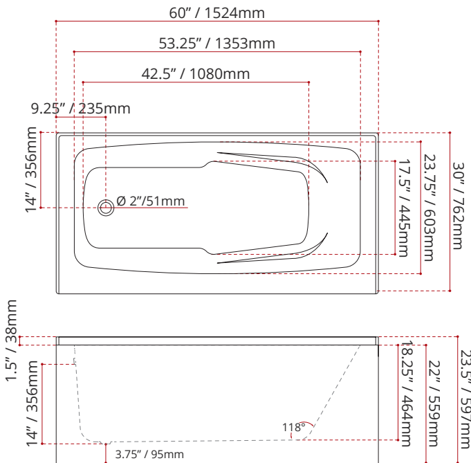
MODEL NUMBER : 5195 (LEFT HAND DRAIN LOCATION)
