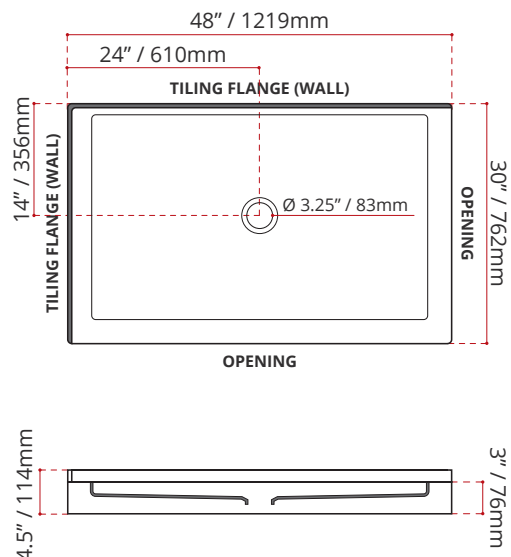
SDTCD4830R1 (RIGHT HAND THRESHOLD OPENING)
