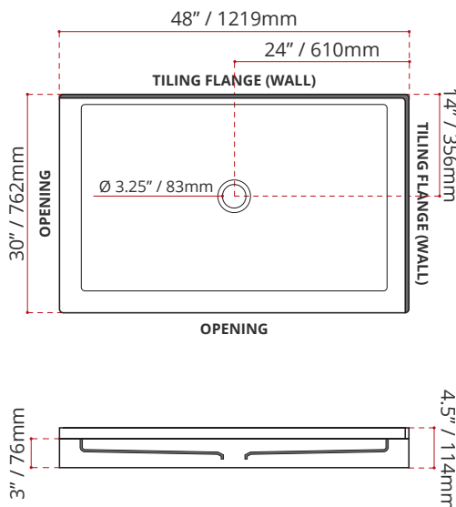
SDTCD4830L1 (LEFT HAND THRESHOLD OPENING)
