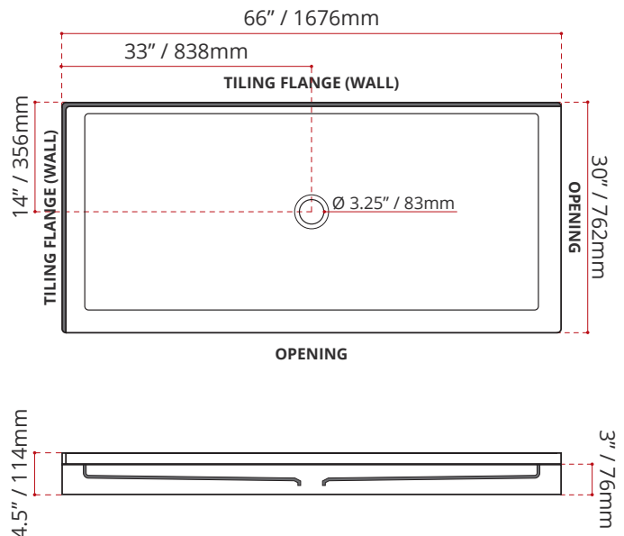
SDTCD6630R4 (RIGHT HAND THRESHOLD OPENING)
