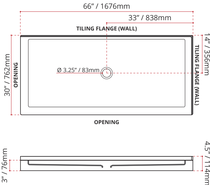
SDTCD6630L4 (LEFT HAND THRESHOLD OPENING)
