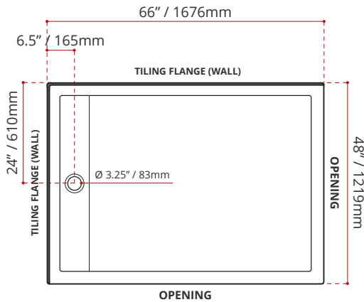
SDTLD6648L1 (LEFT HAND DRAIN LOCATION) (RIGHT HAND THRESHOLD / OPENING)
