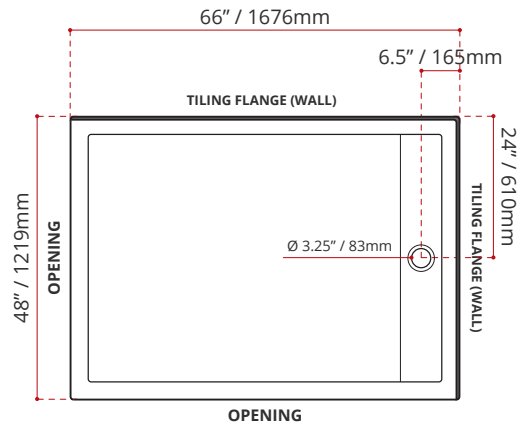
SDTLD6648R1 (RIGHT HAND DRAIN LOCATION) (LEFT HAND THRESHOLD / OPENING)
