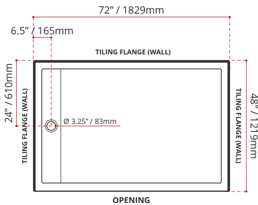
SSTLD7248L1 (LEFT HAND DRAIN LOCATION)
