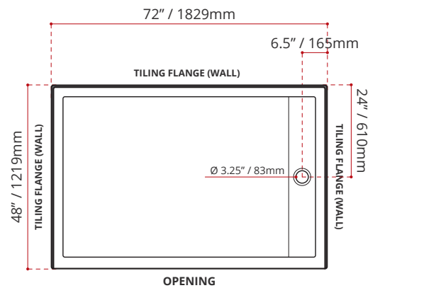
SSTLD7248R1 (RIGHT HAND DRAIN LOCATION)
