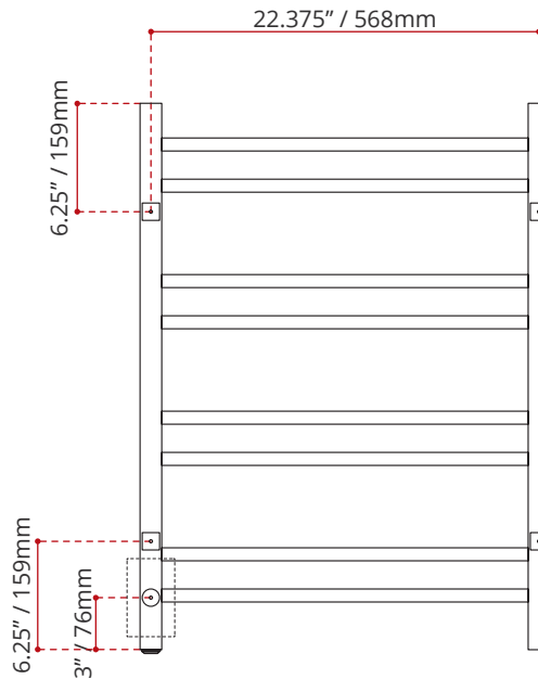
BACK VIEW
